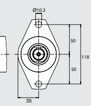
Stainless steel Flange Ordering No. 4430 2357 80
