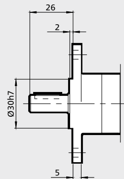
Flange Ordering No. 4110 0984 85 with holes 4110 0984 80 without holes
