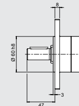
Stainless steel Flange Ordering No. 4430 2357 80
