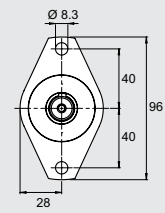
Stainless steel Flange Ordering No. 4430 1483 80
