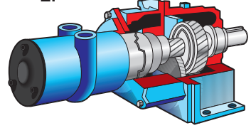
Planetary gear (1), helical gear (2).
